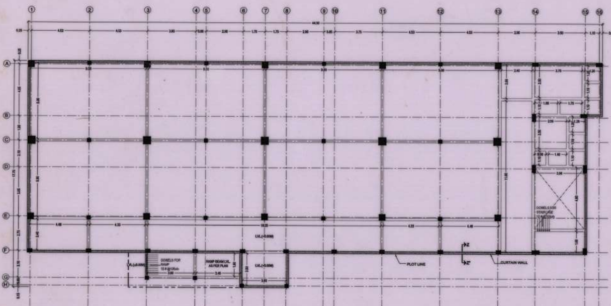
CURTAIN WALL PLAN
